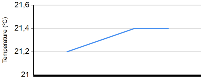
Air Temperature
