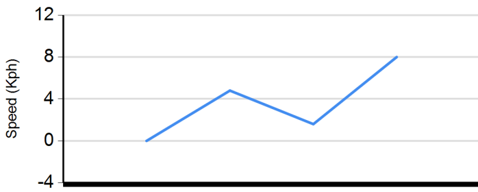
Wind Speed
